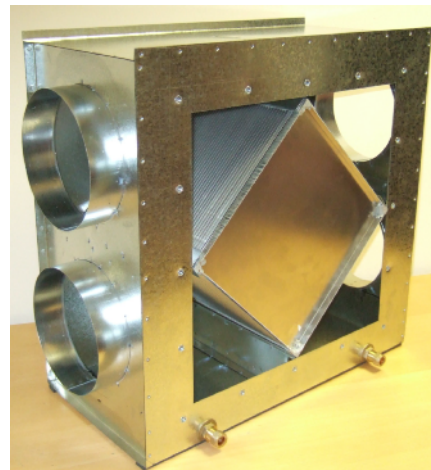
Plenum box with access cover removed
