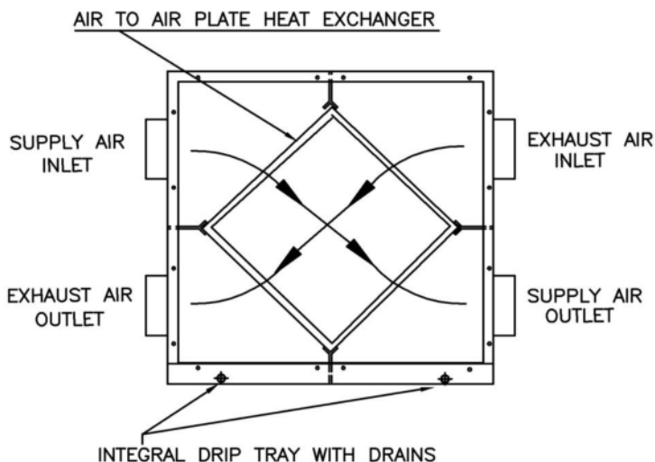
Plenum box with access cover removed
