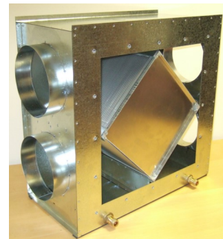
Plenum box with access cover removed
