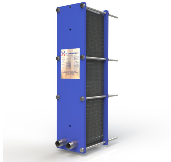
Single section heat exchanger with painted steel frame & BSP male connections
